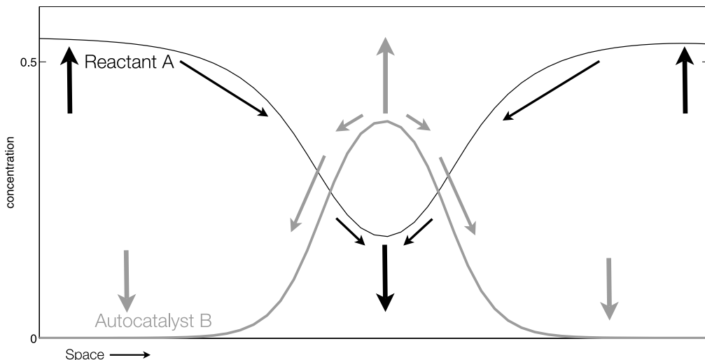
Figure 2. Concentration profile of a spot: a precarious, individuated dissipative structure found in the Gray-Scott reaction-diffusion system. For clarity of display a one-dimensional version of the system is shown. The spatially individuated structure of the spot remains constant over time due to a precarious balance between reaction and diffusion processes. The arrows indicate the direction in which processes occur. For example, near the center of the spot, B is continually produced by the autocatalytic reaction (upward arrow in the middle), but its concentration there remains constant due to the diffusive transport of B toward the sides of the spot (angled arrows). This diffusion is in turn balanced by the tendency for the autocatalyst to decay away in the regions where its concentration is low, that is, outside the center of the spot (downward arrows). (Figure taken from Virgo [107, p. 86].)
