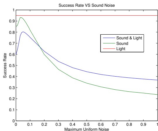
Figure 8: Comparison between the performance of each condition (light only, sound only and both) with different levels of noise on the sound module.
