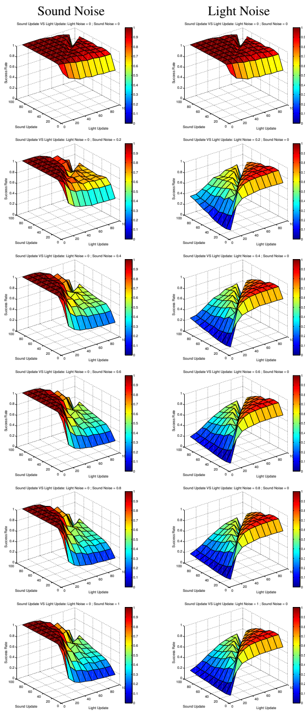
Figure 6: Variation of the performance of the robot under different timescales and different level of noise for the sensory modules. From top to bottom, the level of uniform noise is varied from 0 to 1 by increment of 0.2. The left column has noise on the sound sensor only, while the right one has noise on the light sensor only.
